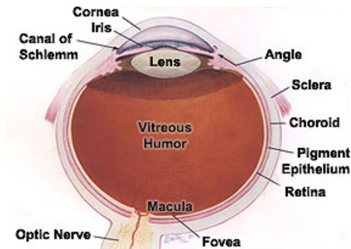
Figure 2.1: Eye Components
