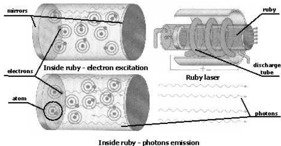
Figure 1.1: Ruby Laser
