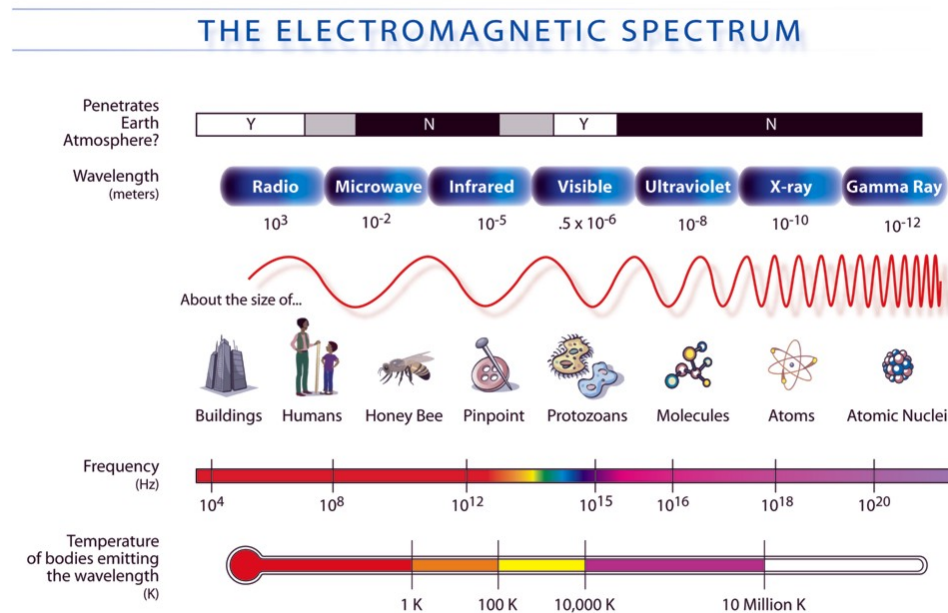
Figure 1: Electromagnetic Spectrum
